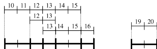
Fig. 4. Evaluation of fragments of the set of time intervals \{[10,15], [12,13], [13,16], [19,20]\} . The result (shown in bold in the figure) is the set \{[10,12), [12,13), [13,13], (13,15), (15,16), [19,20]\} .
